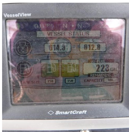
Vessel View Digital Smartcraft Monitor
